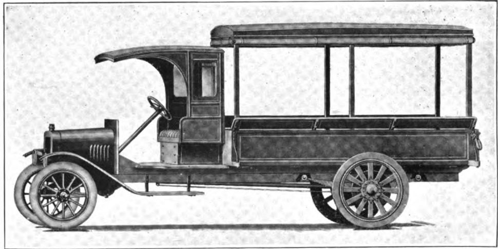
NEW TYPE EXPRESS BODY ON A FORM-A-TRUCK CHASSIS Built by the Columbia (Pa.) Wagon Co.
